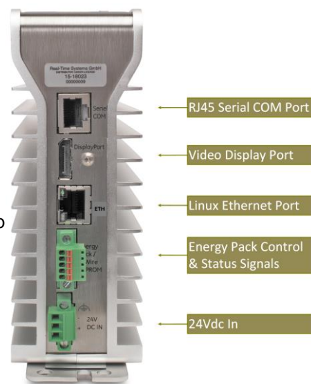
Figure 4: Underside Ports & Connectors 47
