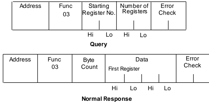
Figure 59: RTU Read Registers Message Format
