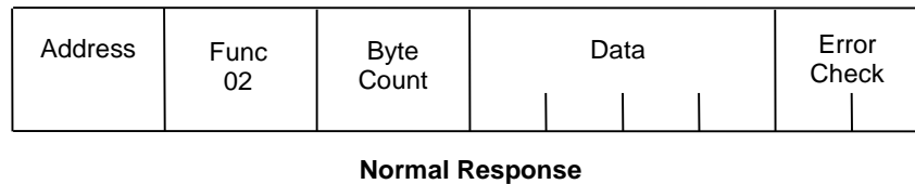
Figure 58: RTU Read Input Table Message Format
