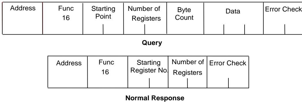
Figure 66: RTU Preset Multiple Registers Message Format
