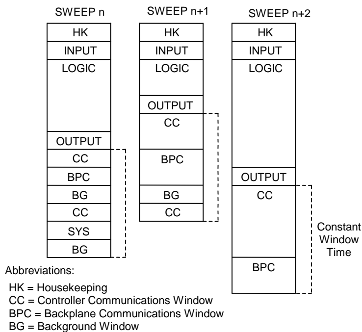
Figure 48: Typical Sweeps in Constant Window Mode
