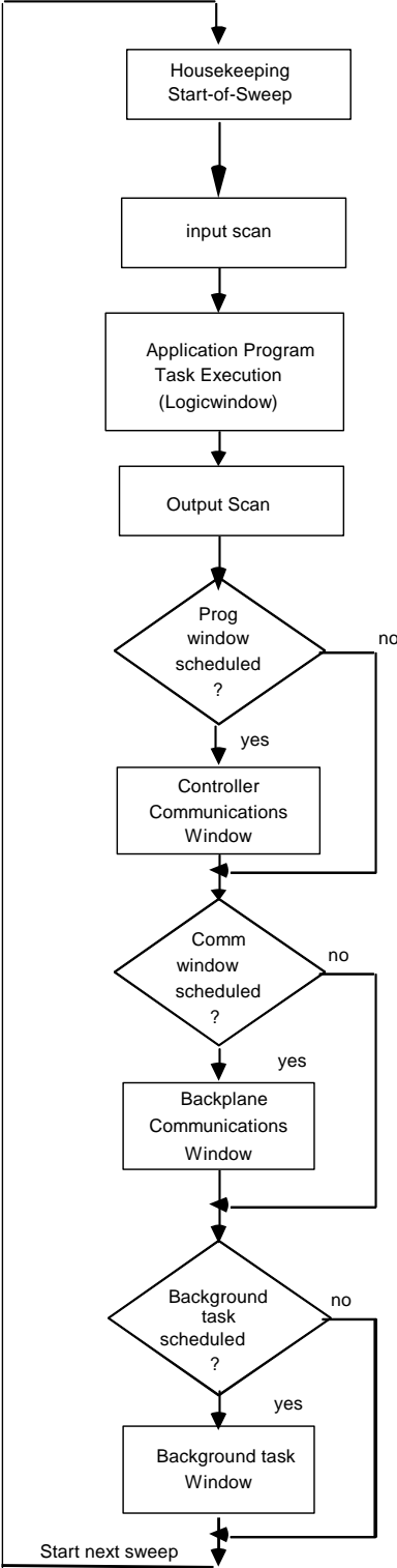
Figure 45: Major Phases of a Typical CPU Sweep
