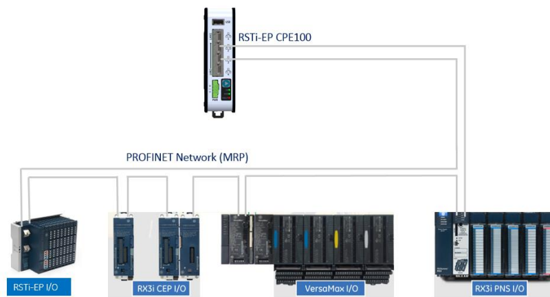
Figure 40: Typical Multi-Tier LAN Application (Ring Topology)
