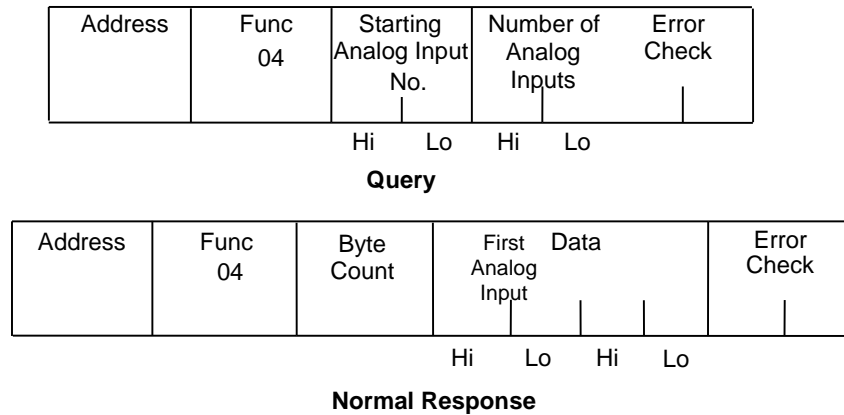
Figure 60: RTU Read Analog Inputs Message Format
