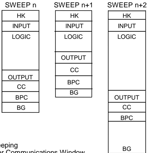
Figure 46: Typical Sweeps in Normal Sweep Mode
