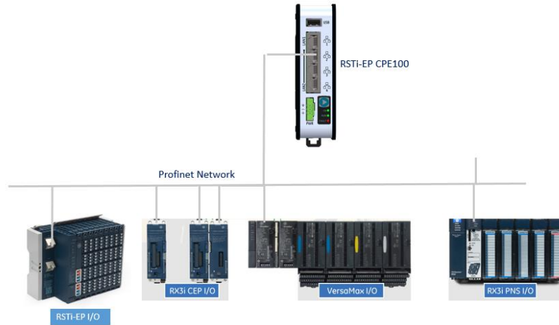
Figure 39: Typical Multi-Tier LAN Application (Star/Bus Topology)
